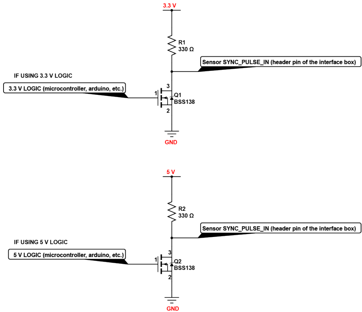
Figure5.1: Example Circuits for 3.3 V and 5 V logic
