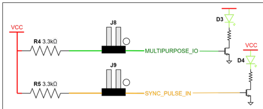
Figure 7.4: J8 & J9 Circuitry
