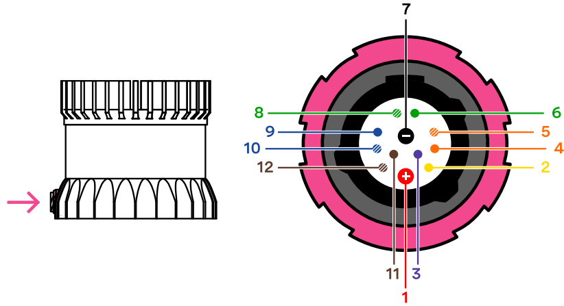
Figure7.1: cable pinout of on-sensor receptacle
