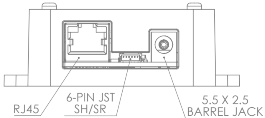
Figure7.7: Connector Outline
