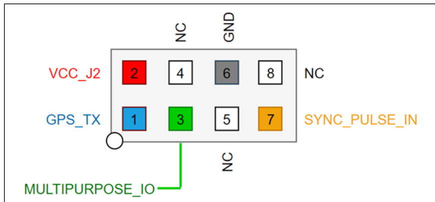
Figure7.5: J7 Circuitry
