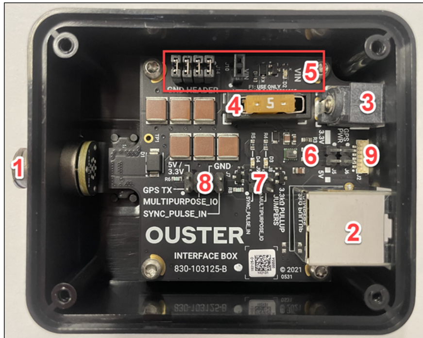
Figure 7.3: Components
