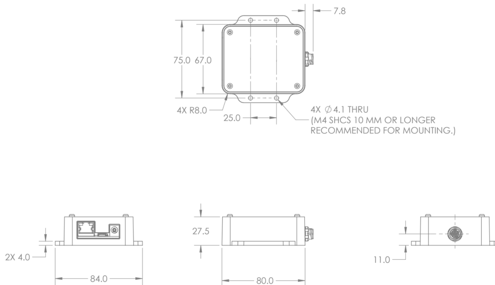
Figure 7.8: Mounting Guidelines - Ibox
