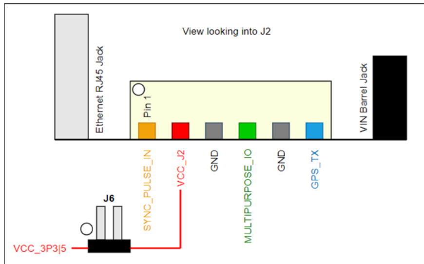
Figure7.6: J2 Circuitry
