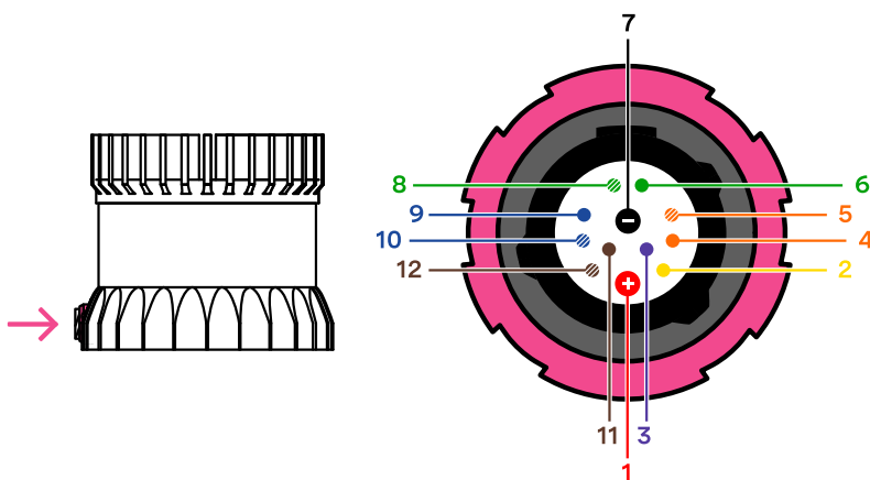
Figure4.1: cable pinout of on-sensor receptacle
